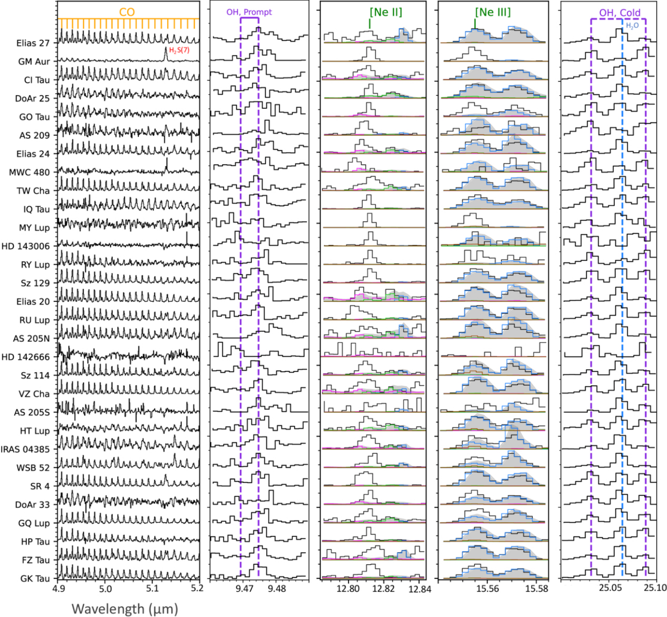
Figure 5. from Nicole Arulanantham et al 2025 Astron. J. 170 doi:10.3847/1538-3881/addd01 https://dx.doi.org/10.3847/1538-3881/addd01 © 2025. The Author(s). Published by the American Astronomical Society.
