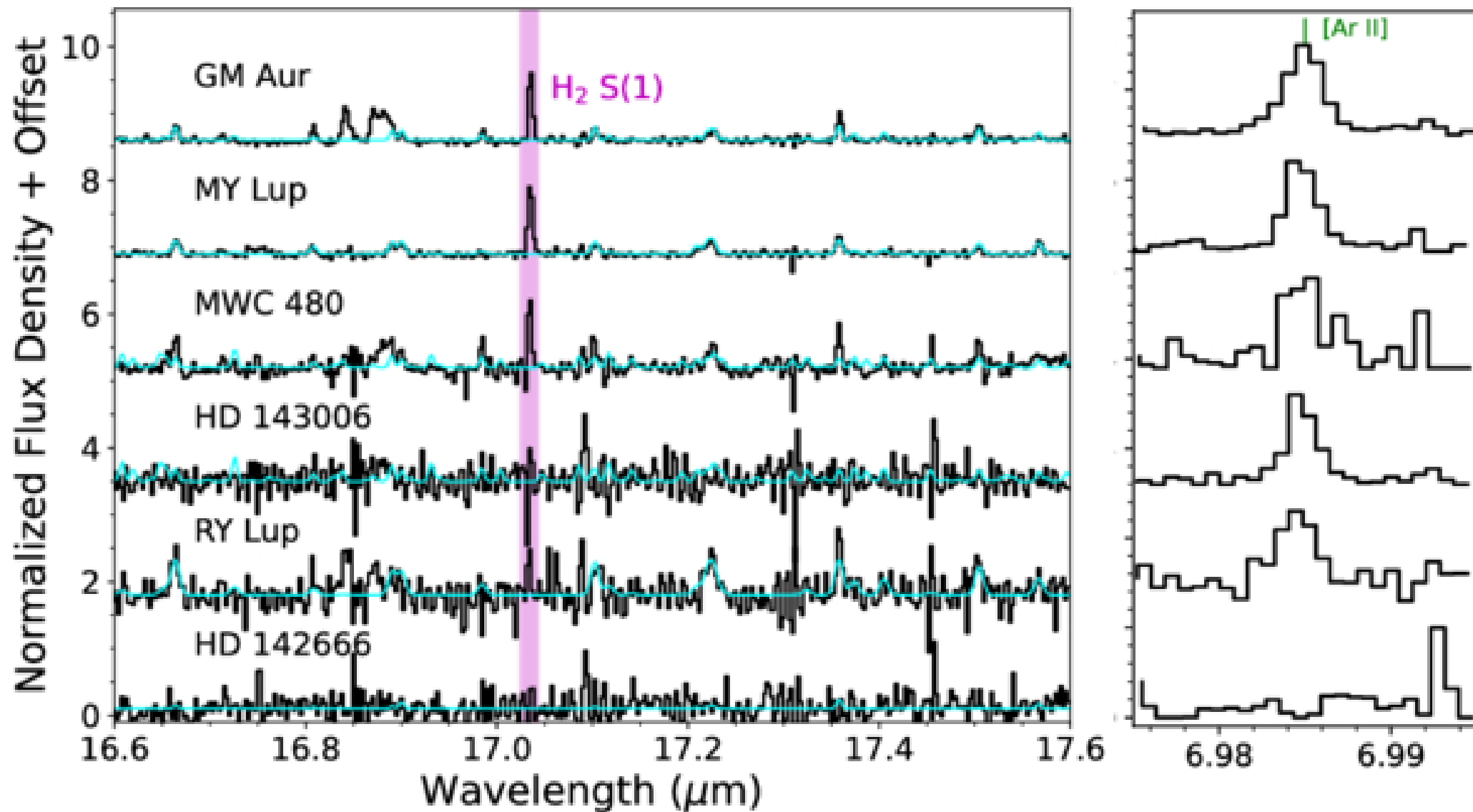
Figure A1. from Nicole Arulanantham et al 2025 Astron. J. 170 doi:10.3847/1538-3881/addd01 https://dx.doi.org/10.3847/1538-3881/addd01 © 2025. The Author(s). Published by the American Astronomical Society.
