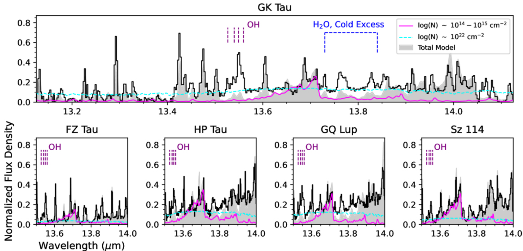
Figure 18. from Nicole Arulanantham et al 2025 Astron. J. 170 doi:10.3847/1538-3881/addd01 https://dx.doi.org/10.3847/1538-3881/addd01 © 2025. The Author(s). Published by the American Astronomical Society.
