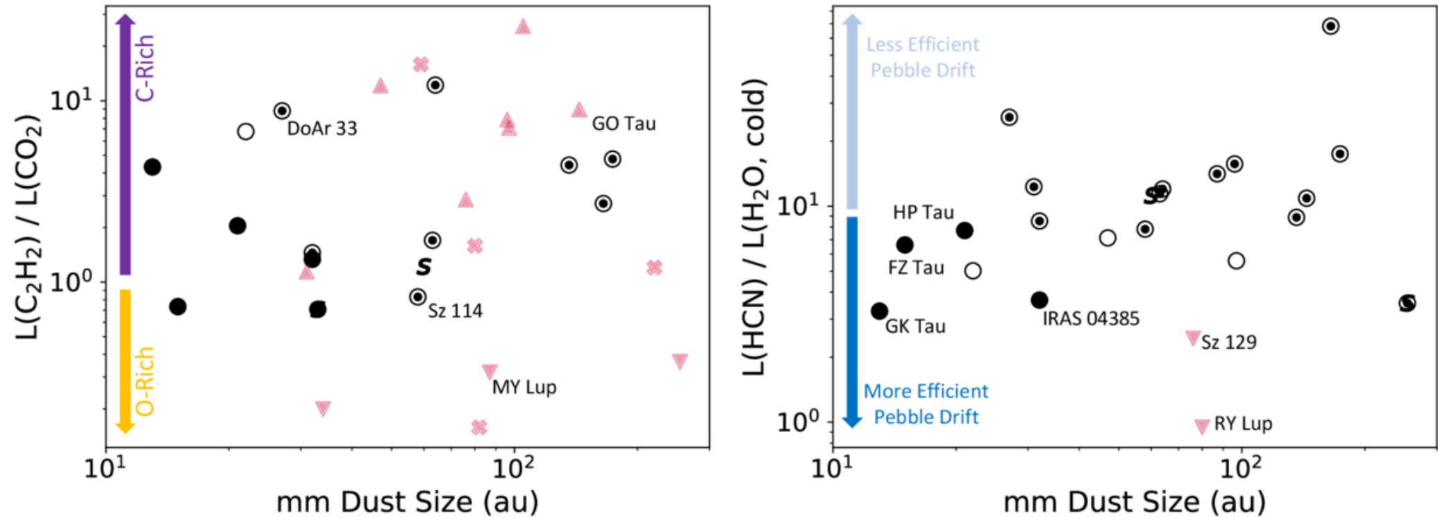
Figure 17. from Nicole Arulanantham et al 2025 Astron. J. 170 doi:10.3847/1538-3881/addd01 https://dx.doi.org/10.3847/1538-3881/addd01 © 2025. The Author(s). Published by the American Astronomical Society.
