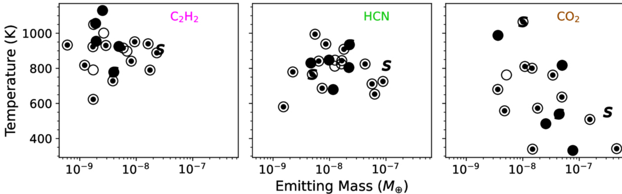
Figure 14. from Nicole Arulanantham et al 2025 Astron. J. 170 doi:10.3847/1538-3881/addd01 https://dx.doi.org/10.3847/1538-3881/addd01 © 2025. The Author(s). Published by the American Astronomical Society.
