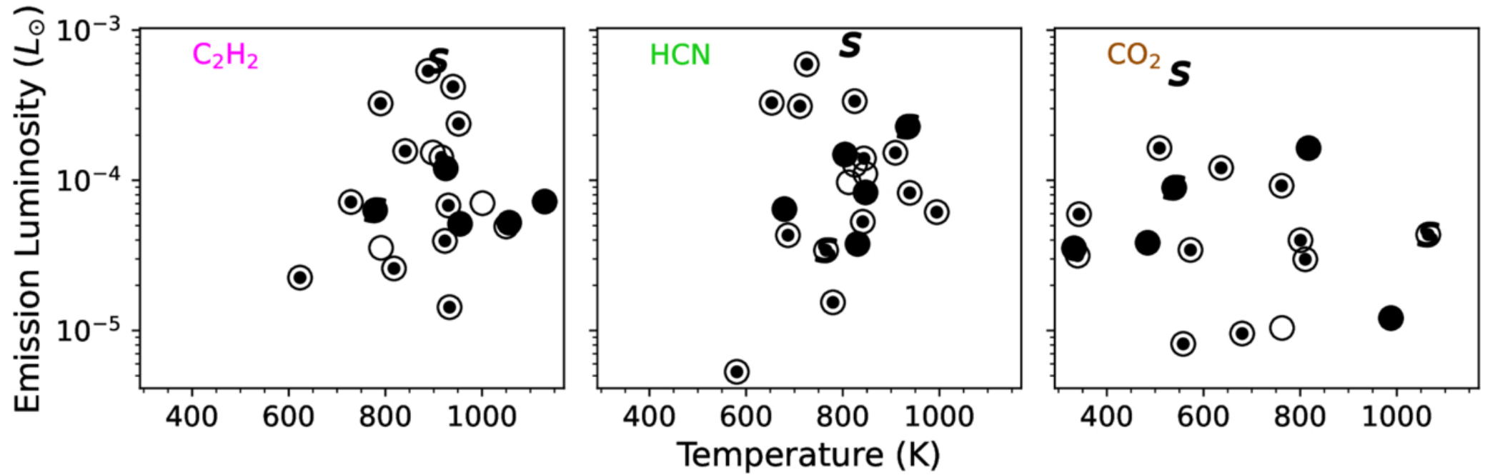
Figure 12. from Nicole Arulanantham et al 2025 Astron. J. 170 doi:10.3847/1538-3881/addd01 https://dx.doi.org/10.3847/1538-3881/addd01 © 2025. The Author(s). Published by the American Astronomical Society.
