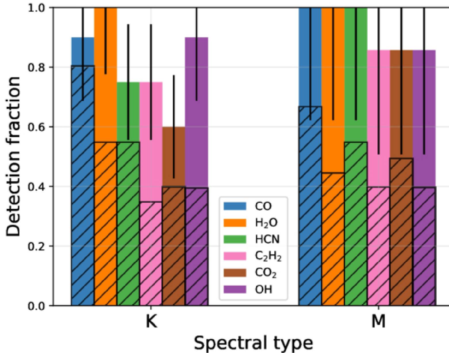
Figure 11. from Nicole Arulanantham et al 2025 Astron. J. 170 doi:10.3847/1538-3881/addd01 https://dx.doi.org/10.3847/1538-3881/addd01 © 2025. The Author(s). Published by the American Astronomical Society.
