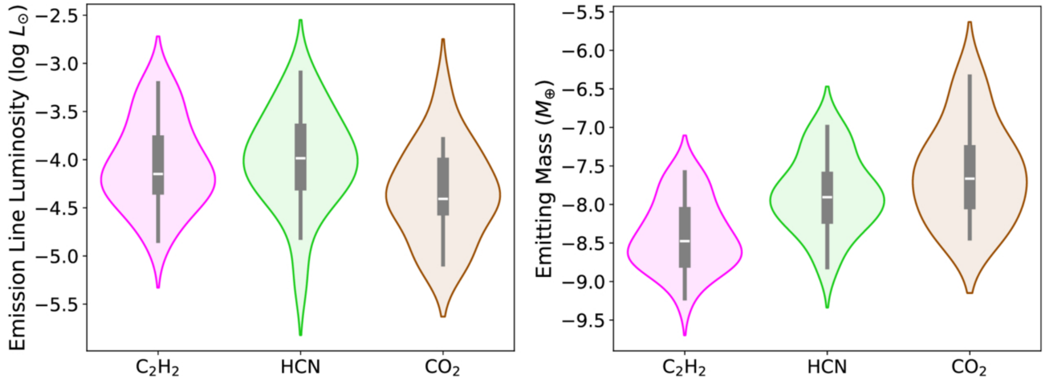
Figure 10. from Nicole Arulanantham et al 2025 Astron. J. 170 doi:10.3847/1538-3881/addd01 https://dx.doi.org/10.3847/1538-3881/addd01 © 2025. The Author(s). Published by the American Astronomical Society.
