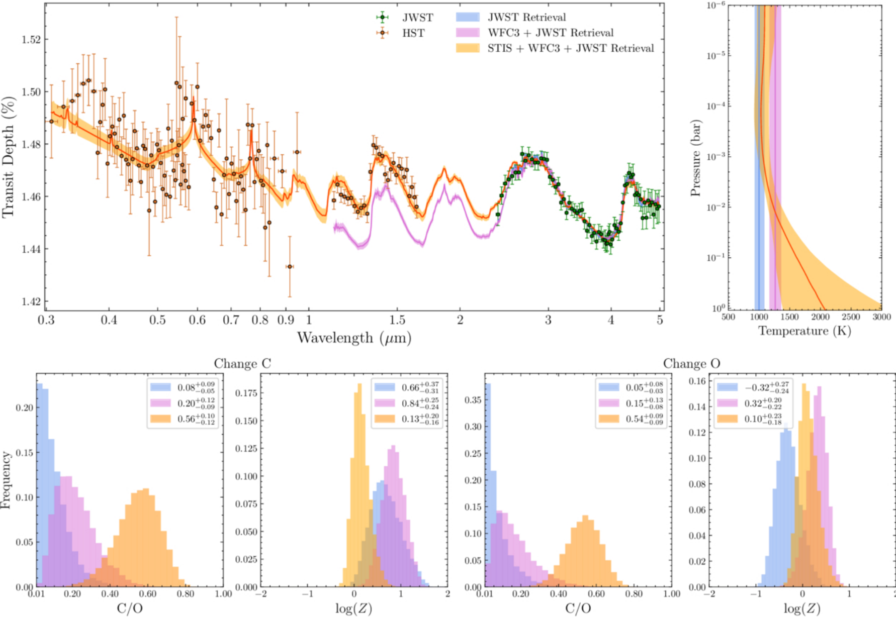
Figure 9. from Avinash Verma et al 2025 Astron. J. 170 doi:10.3847/1538-3881/addc5c https://dx.doi.org/10.3847/1538-3881/addc5c © 2025. The Author(s). Published by the American Astronomical Society.
