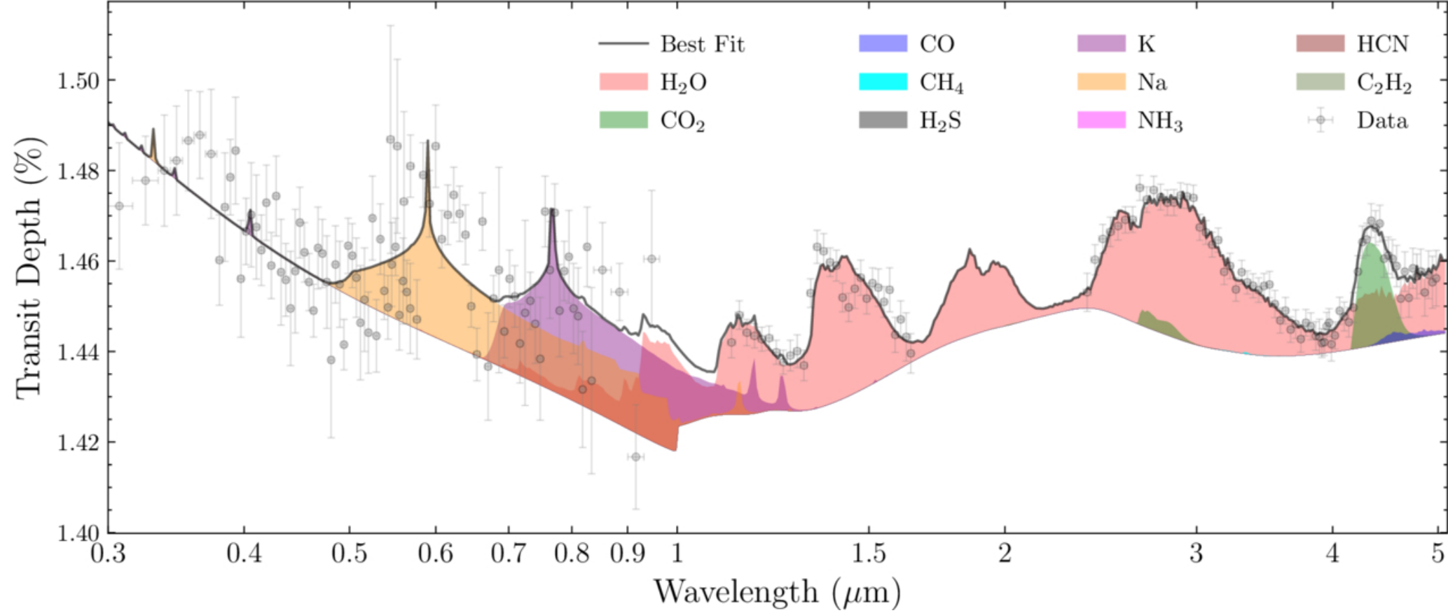
Figure 8. from Avinash Verma et al 2025 Astron. J. 170 doi:10.3847/1538-3881/addc5c https://dx.doi.org/10.3847/1538-3881/addc5c © 2025. The Author(s). Published by the American Astronomical Society.
