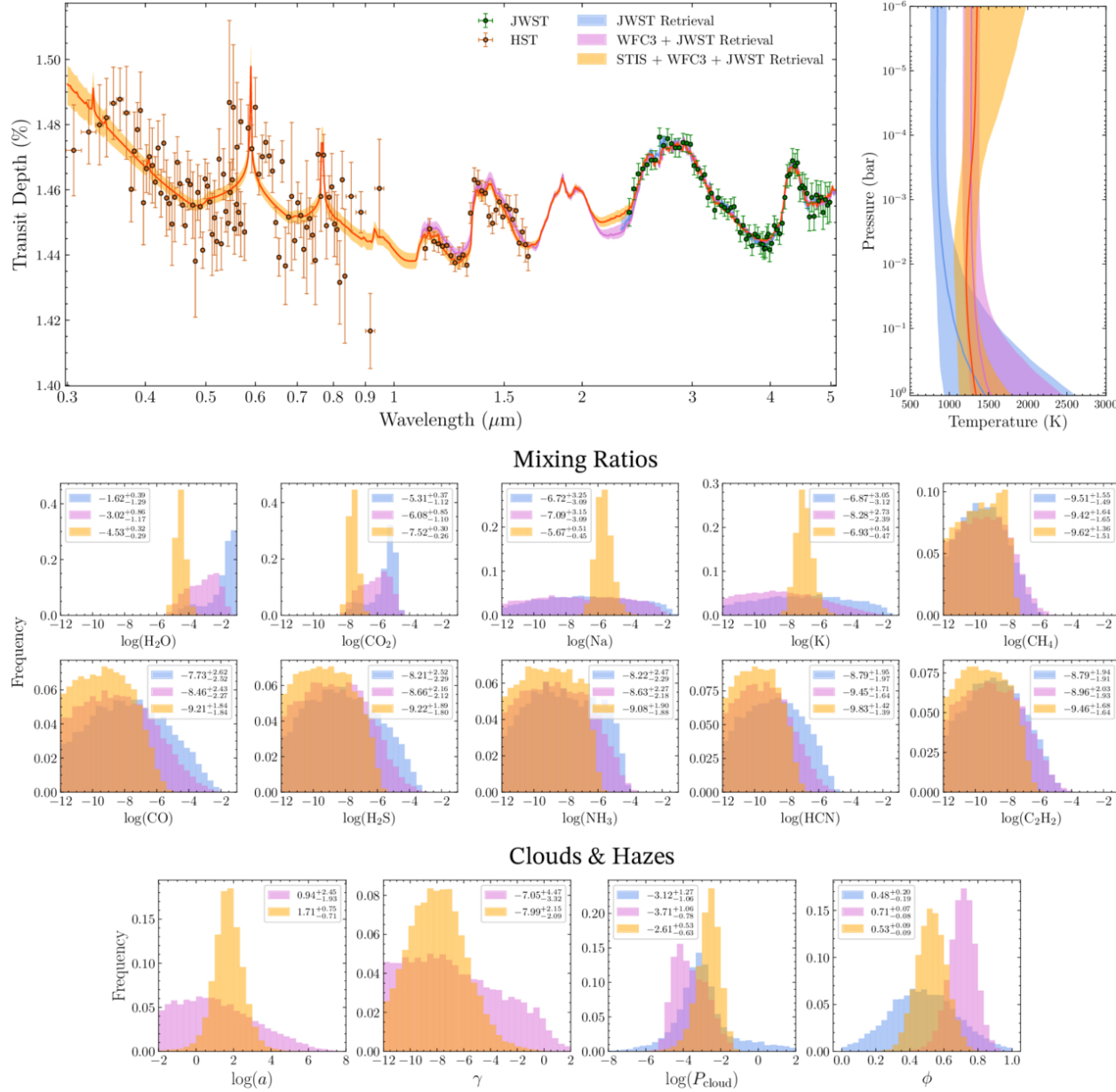
Figure 7. from Avinash Verma et al 2025 Astron. J. 170 doi:10.3847/1538-3881/addc5c https://dx.doi.org/10.3847/1538-3881/addc5c © 2025. The Author(s). Published by the American Astronomical Society.
