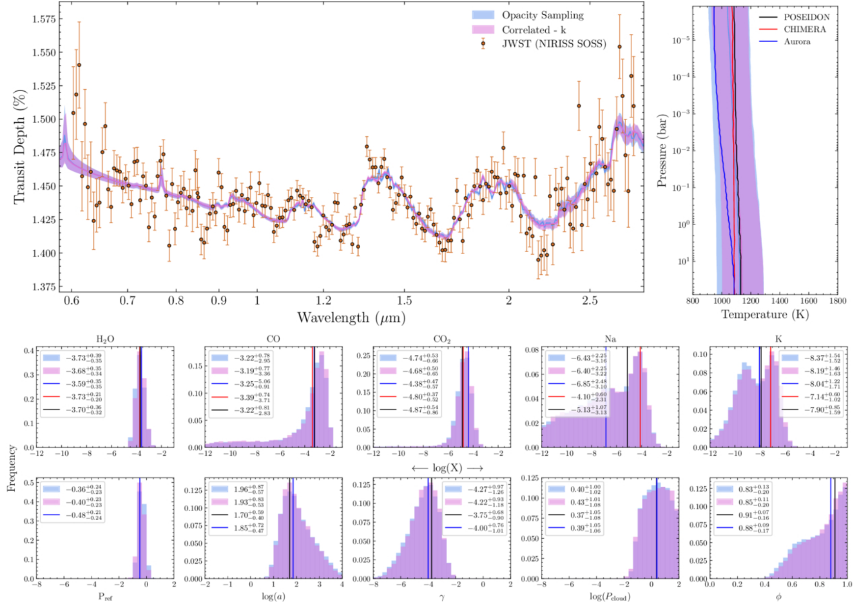
Figure 6. from Avinash Verma et al 2025 Astron. J. 170 doi:10.3847/1538-3881/addc5c https://dx.doi.org/10.3847/1538-3881/addc5c © 2025. The Author(s). Published by the American Astronomical Society.
