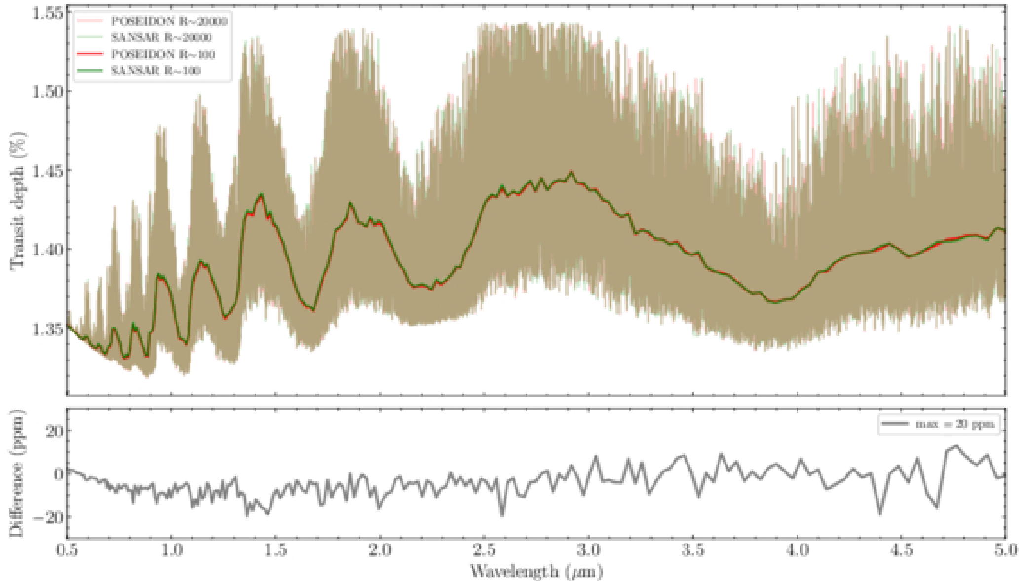
Figure 4. from Avinash Verma et al 2025 Astron. J. 170 doi:10.3847/1538-3881/addc5c https://dx.doi.org/10.3847/1538-3881/addc5c © 2025. The Author(s). Published by the American Astronomical Society.
