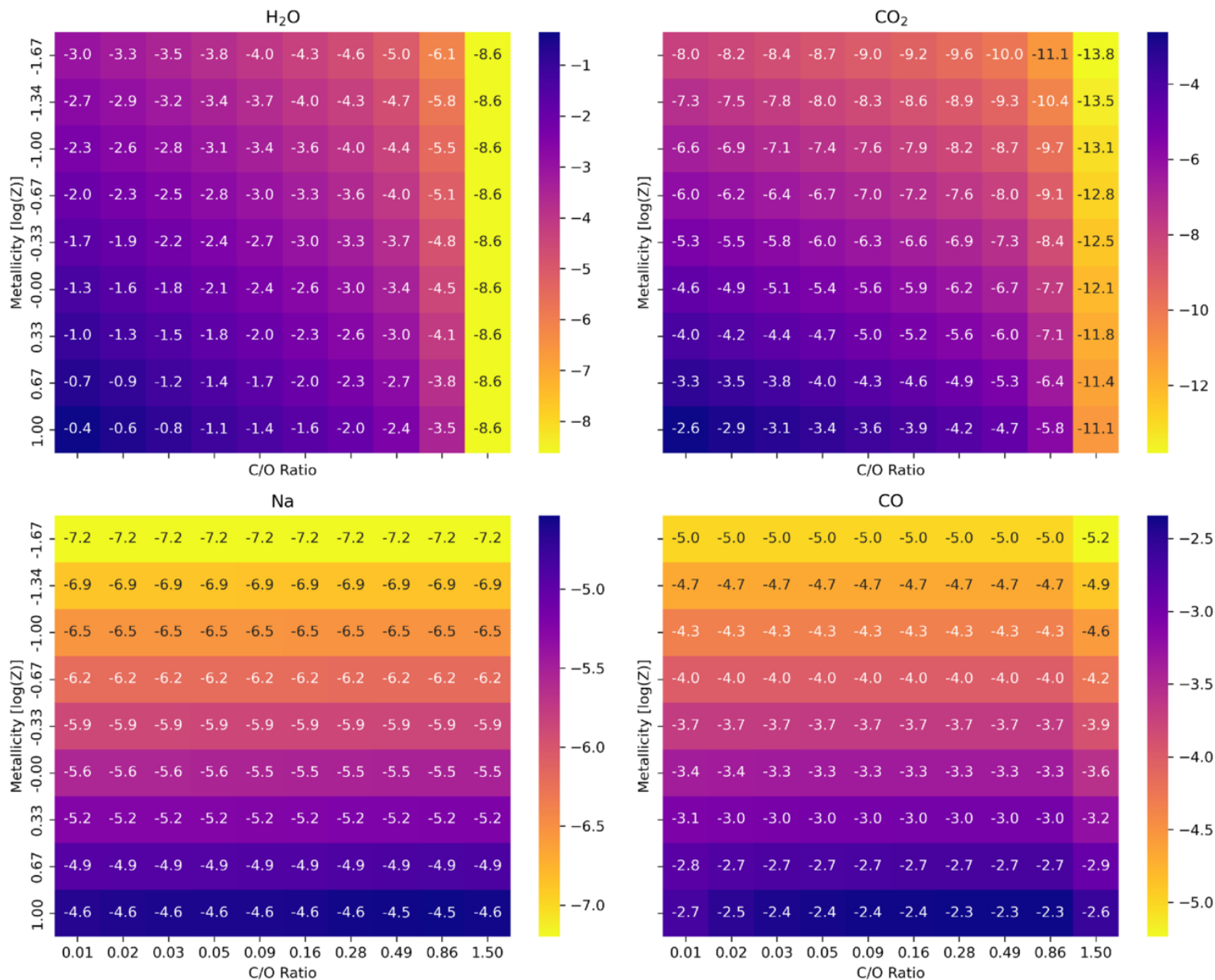
Figure 20. from Avinash Verma et al 2025 Astron. J. 170 doi:10.3847/1538-3881/addc5c https://dx.doi.org/10.3847/1538-3881/addc5c © 2025. The Author(s). Published by the American Astronomical Society.
