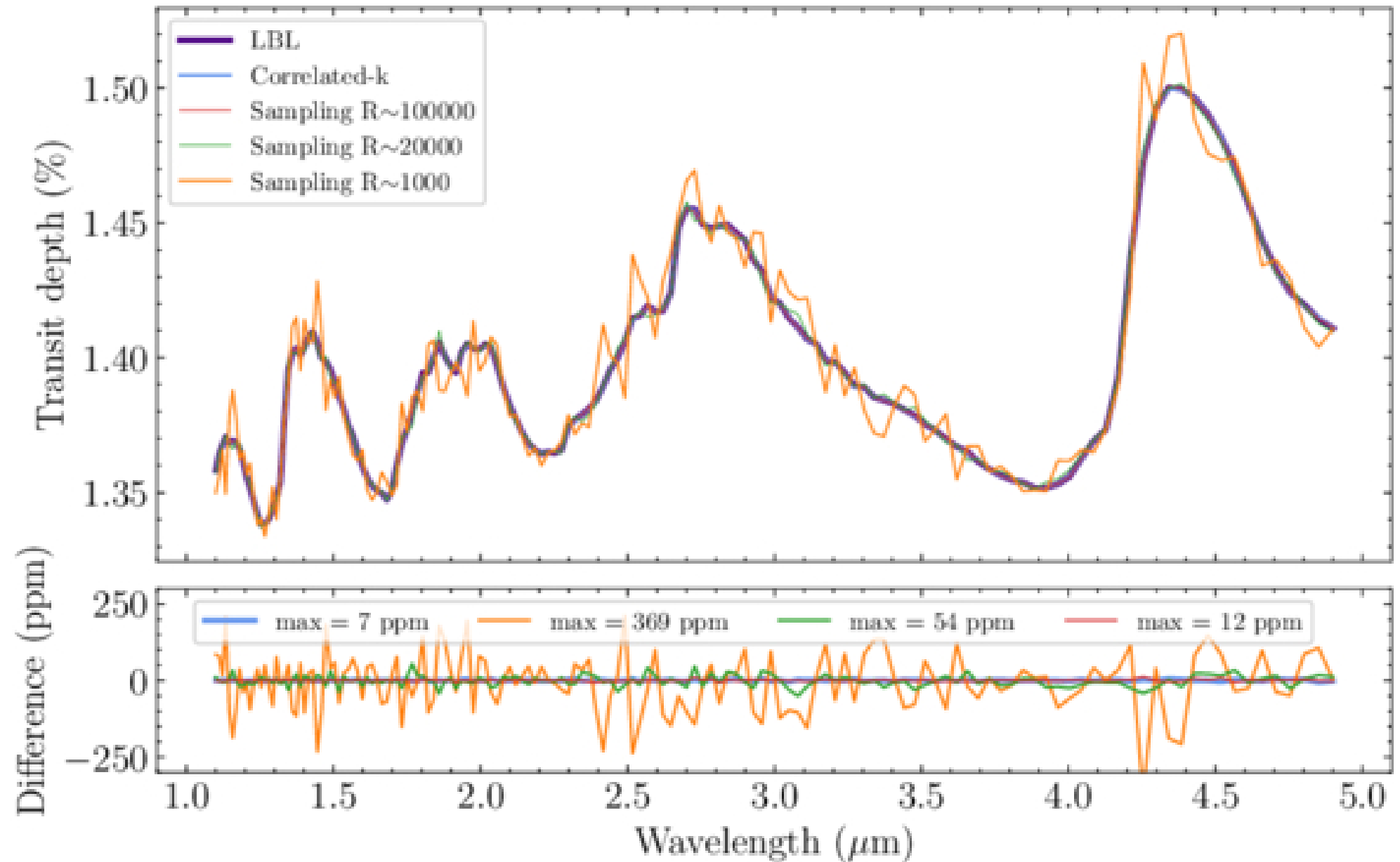
Figure 2. from Avinash Verma et al 2025 Astron. J. 170 doi:10.3847/1538-3881/addc5c https://dx.doi.org/10.3847/1538-3881/addc5c © 2025. The Author(s). Published by the American Astronomical Society.
