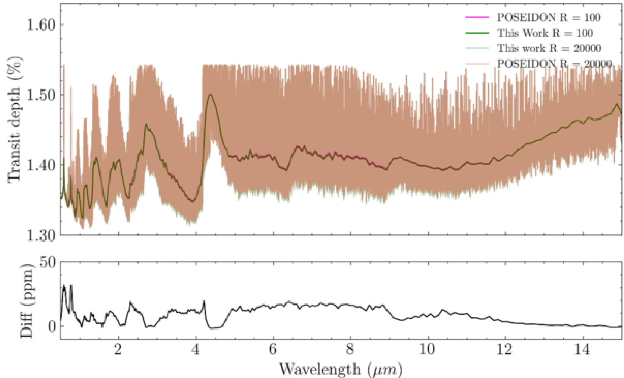
Figure 15. from Avinash Verma et al 2025 Astron. J. 170 doi:10.3847/1538-3881/addc5c https://dx.doi.org/10.3847/1538-3881/addc5c © 2025. The Author(s). Published by the American Astronomical Society.
