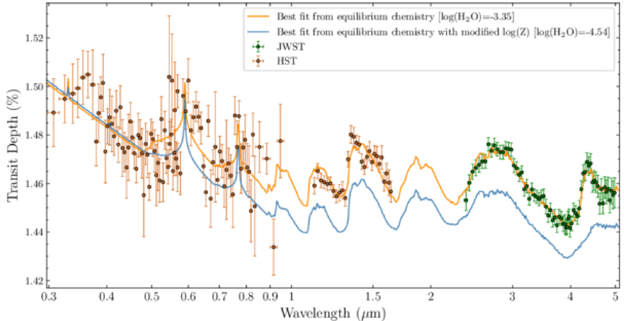
Figure 12. from Avinash Verma et al 2025 Astron. J. 170 doi:10.3847/1538-3881/addc5c https://dx.doi.org/10.3847/1538-3881/addc5c © 2025. The Author(s). Published by the American Astronomical Society.
