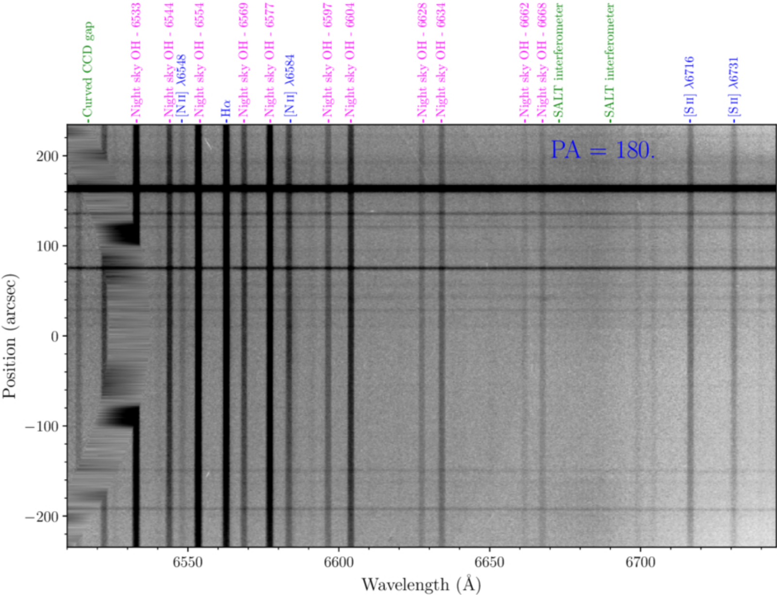
Figure 9. from Michael M. Shara et al 2025 Astron. J. 170 doi:10.3847/1538-3881/addb44 https://dx.doi.org/10.3847/1538-3881/addb44 © 2025. The Author(s). Published by the American Astronomical Society.
