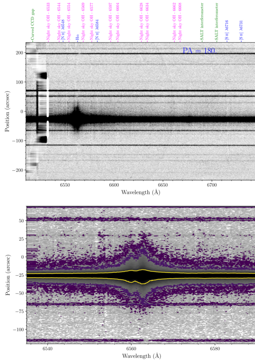
Figure 8. from Michael M. Shara et al 2025 Astron. J. 170 doi:10.3847/1538-3881/addb44 https://dx.doi.org/10.3847/1538-3881/addb44 © 2025. The Author(s). Published by the American Astronomical Society.
