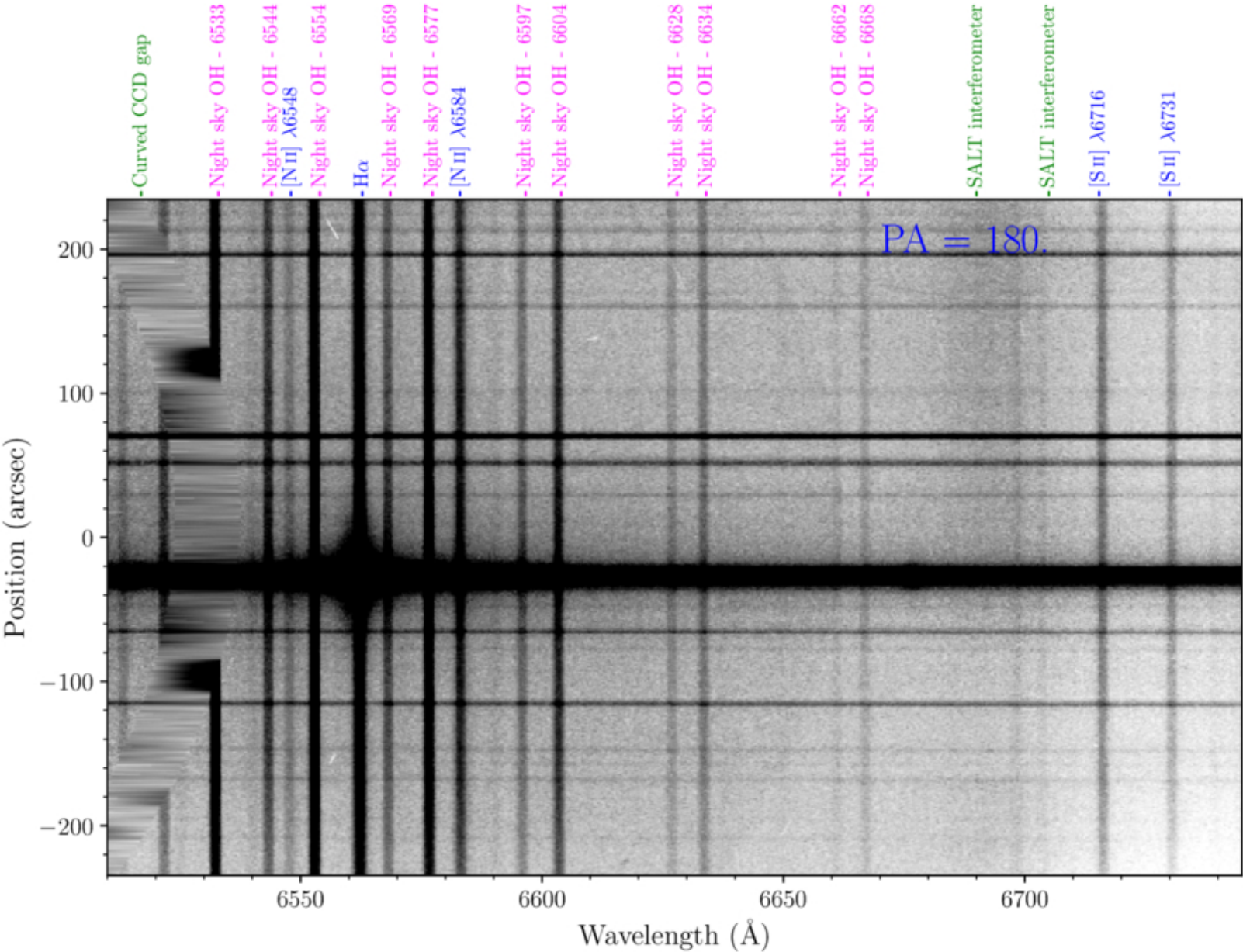
Figure 7. from Michael M. Shara et al 2025 Astron. J. 170 doi:10.3847/1538-3881/addb44 https://dx.doi.org/10.3847/1538-3881/addb44 © 2025. The Author(s). Published by the American Astronomical Society.
