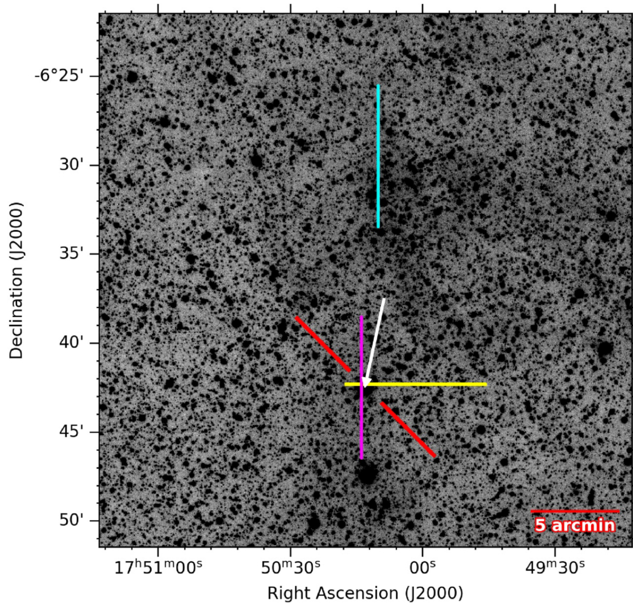
Figure 6. from Michael M. Shara et al 2025 Astron. J. 170 doi:10.3847/1538-3881/addb44 https://dx.doi.org/10.3847/1538-3881/addb44 © 2025. The Author(s). Published by the American Astronomical Society.
