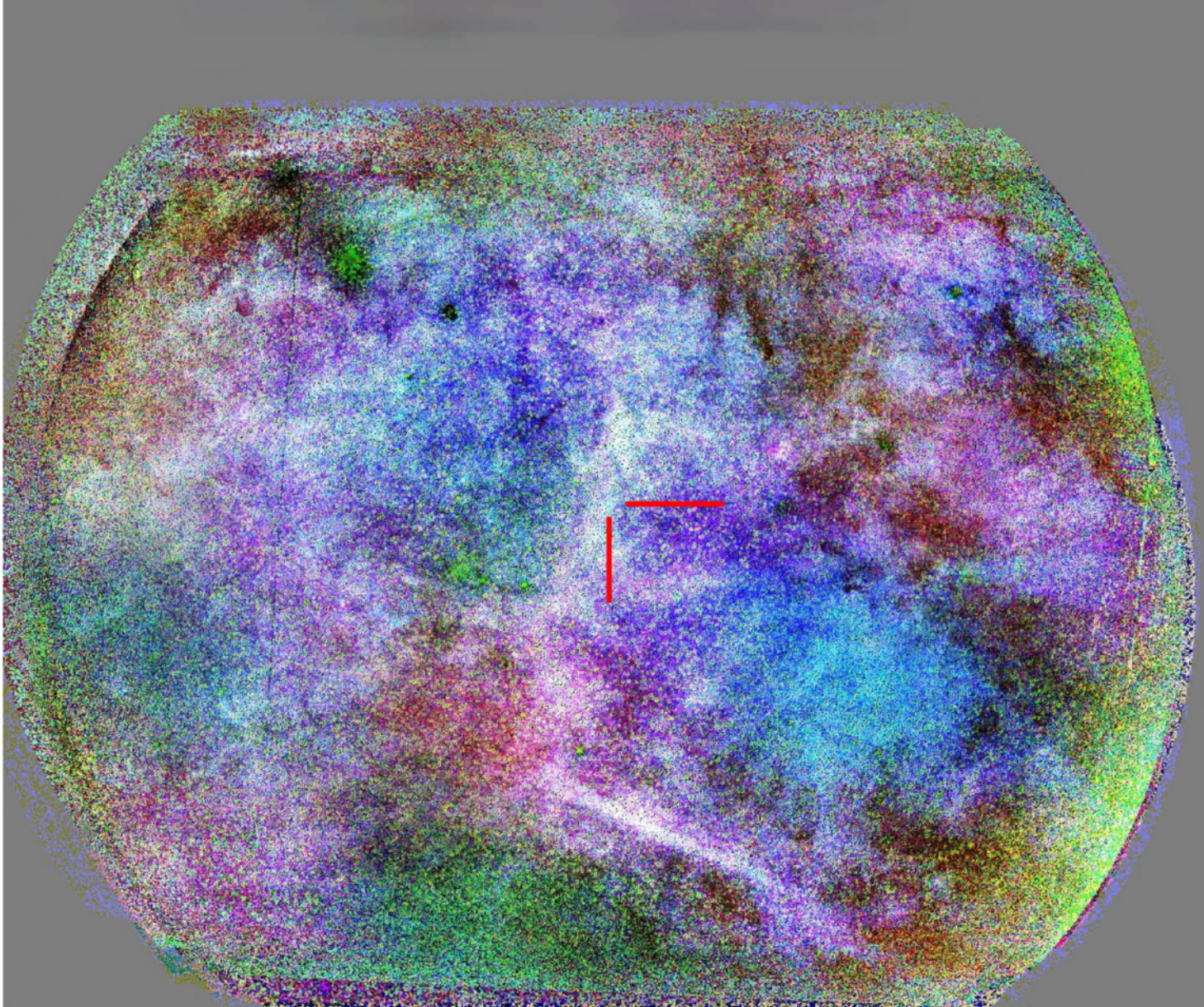
Figure 5. from Michael M. Shara et al 2025 Astron. J. 170 doi:10.3847/1538-3881/addb44 https://dx.doi.org/10.3847/1538-3881/addb44 © 2025. The Author(s). Published by the American Astronomical Society.
