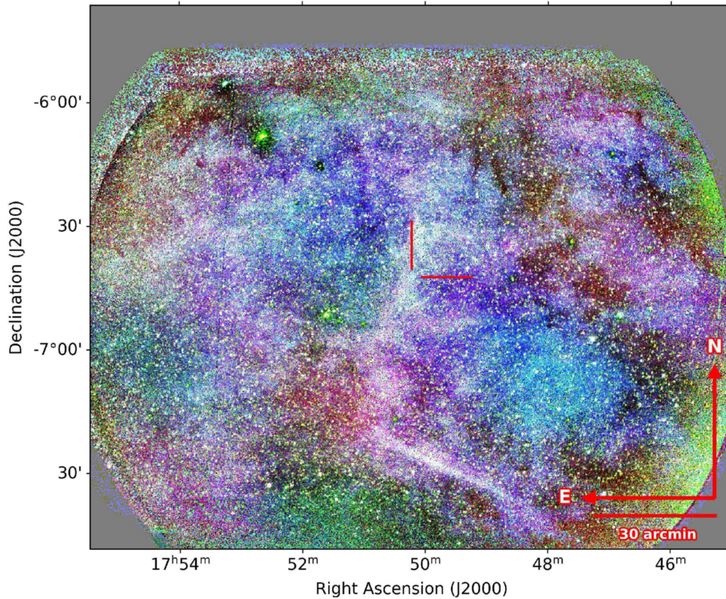
Figure 4. from Michael M. Shara et al 2025 Astron. J. 170 doi:10.3847/1538-3881/addb44 https://dx.doi.org/10.3847/1538-3881/addb44 © 2025. The Author(s). Published by the American Astronomical Society.
