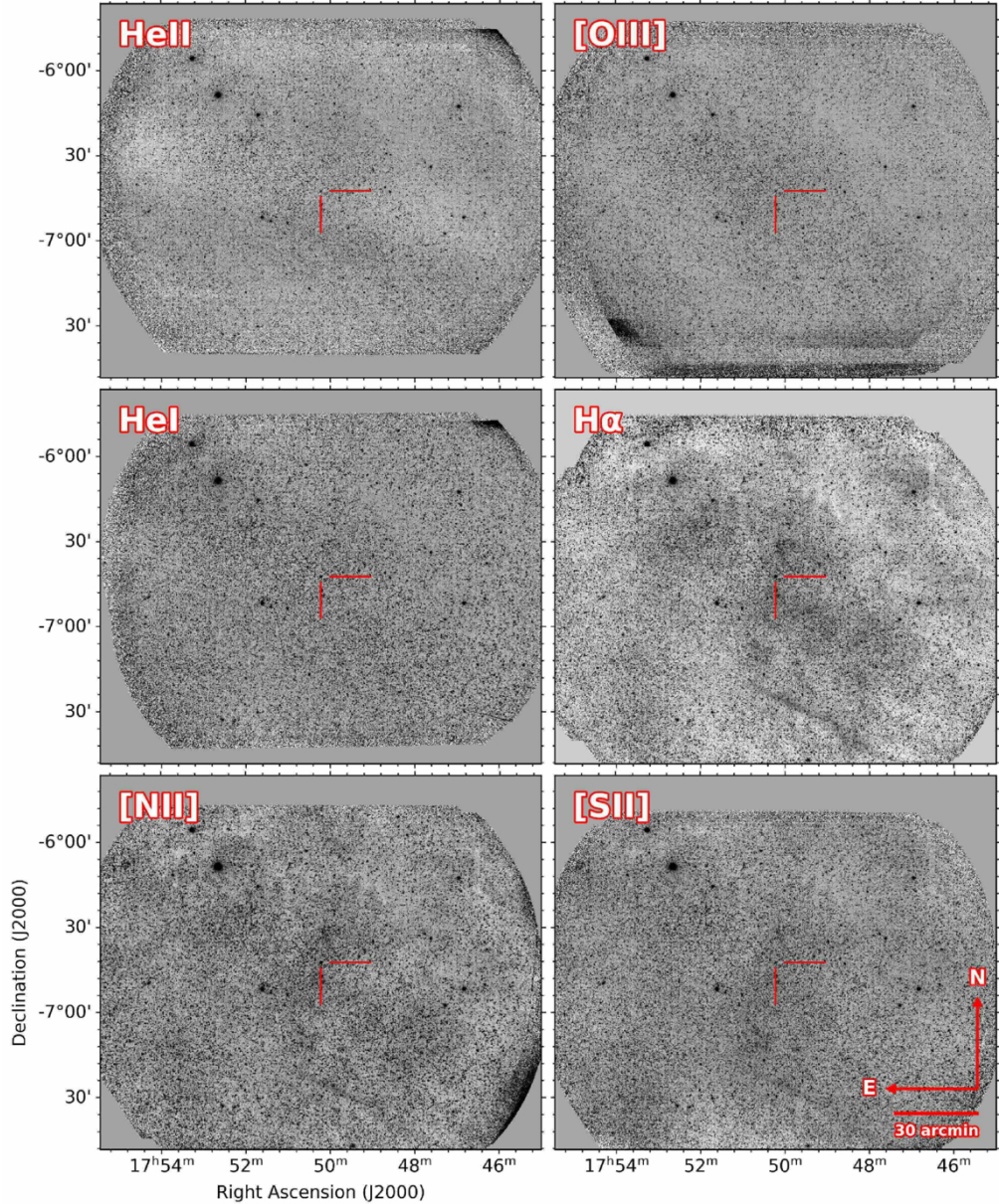
Figure 1. from Michael M. Shara et al 2025 Astron. J. 170 doi:10.3847/1538-3881/addb44 https://dx.doi.org/10.3847/1538-3881/addb44 © 2025. The Author(s). Published by the American Astronomical Society.
