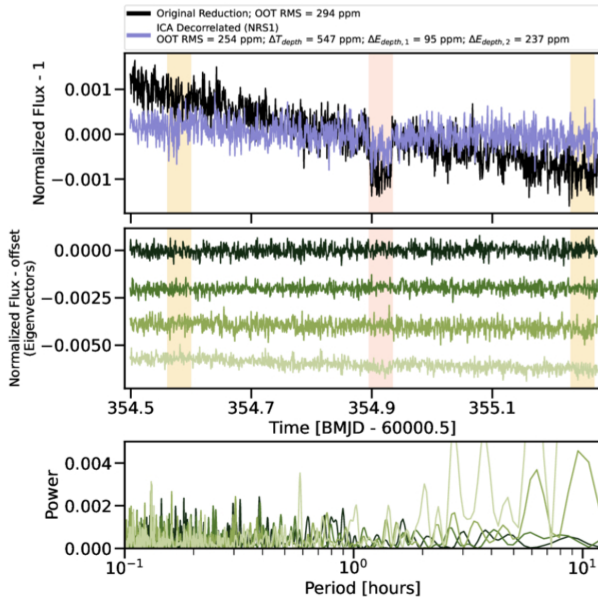
Figure 8. from Rafael Luque et al 2025 Astron. J. 170 doi:10.3847/1538-3881/addb40 https://dx.doi.org/10.3847/1538-3881/addb40 © 2025. The Author(s). Published by the American Astronomical Society.
