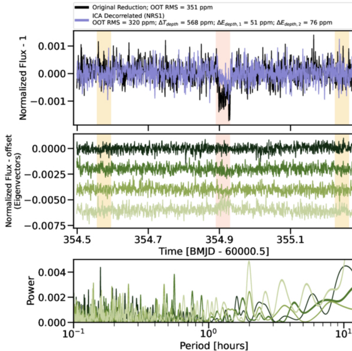
Figure 7. from Rafael Luque et al 2025 Astron. J. 170 doi:10.3847/1538-3881/addb40 https://dx.doi.org/10.3847/1538-3881/addb40 © 2025. The Author(s). Published by the American Astronomical Society.
