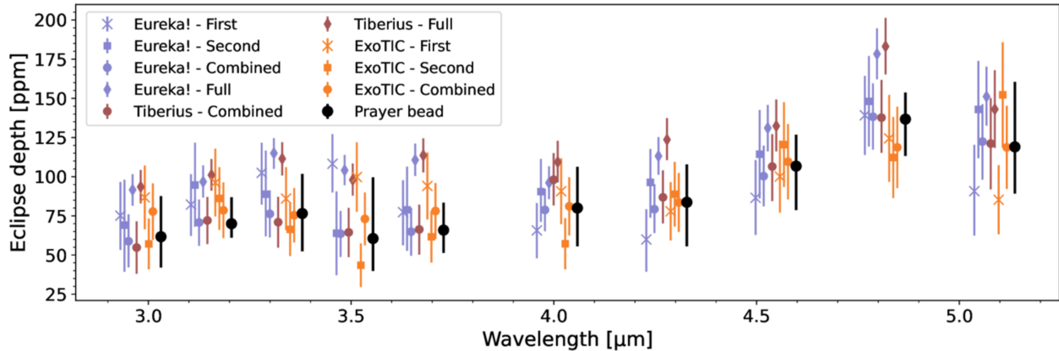
Figure 5. from Rafael Luque et al 2025 Astron. J. 170 doi:10.3847/1538-3881/addb40 https://dx.doi.org/10.3847/1538-3881/addb40 © 2025. The Author(s). Published by the American Astronomical Society.
