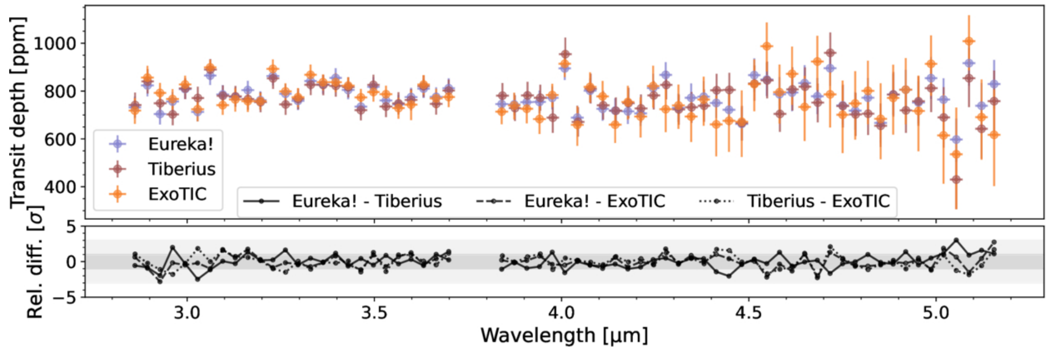
Figure 4. from Rafael Luque et al 2025 Astron. J. 170 doi:10.3847/1538-3881/addb40 https://dx.doi.org/10.3847/1538-3881/addb40 © 2025. The Author(s). Published by the American Astronomical Society.
