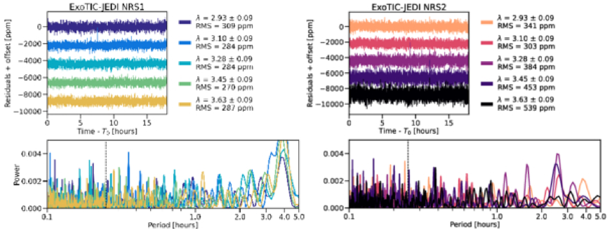
Figure 20. from Rafael Luque et al 2025 Astron. J. 170 doi:10.3847/1538-3881/addb40 https://dx.doi.org/10.3847/1538-3881/addb40 © 2025. The Author(s). Published by the American Astronomical Society.
