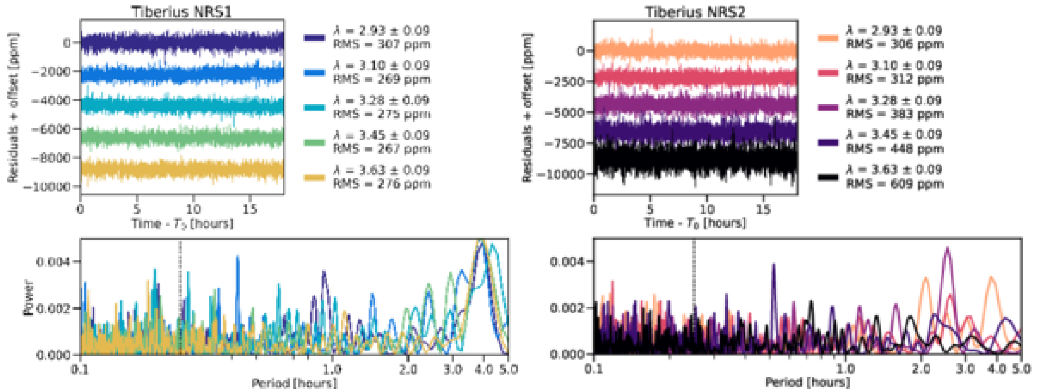
Figure 19. from Rafael Luque et al 2025 Astron. J. 170 doi:10.3847/1538-3881/addb40 https://dx.doi.org/10.3847/1538-3881/addb40 © 2025. The Author(s). Published by the American Astronomical Society.
