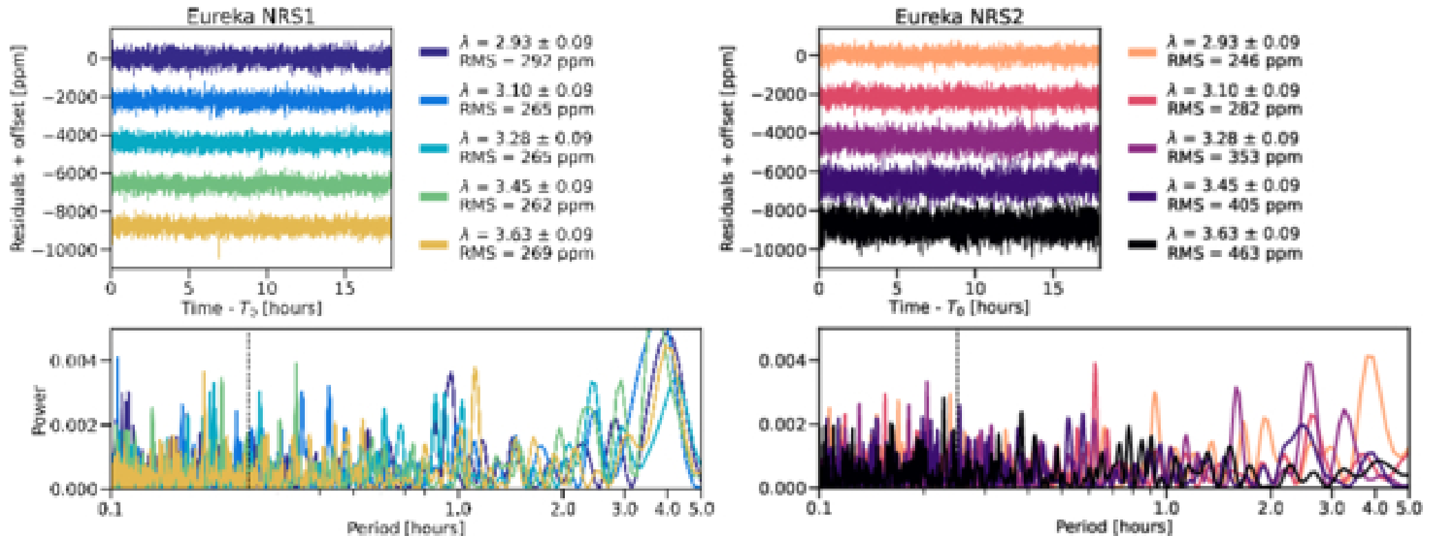
Figure 18. from Rafael Luque et al 2025 Astron. J. 170 doi:10.3847/1538-3881/addb40 https://dx.doi.org/10.3847/1538-3881/addb40 © 2025. The Author(s). Published by the American Astronomical Society.
