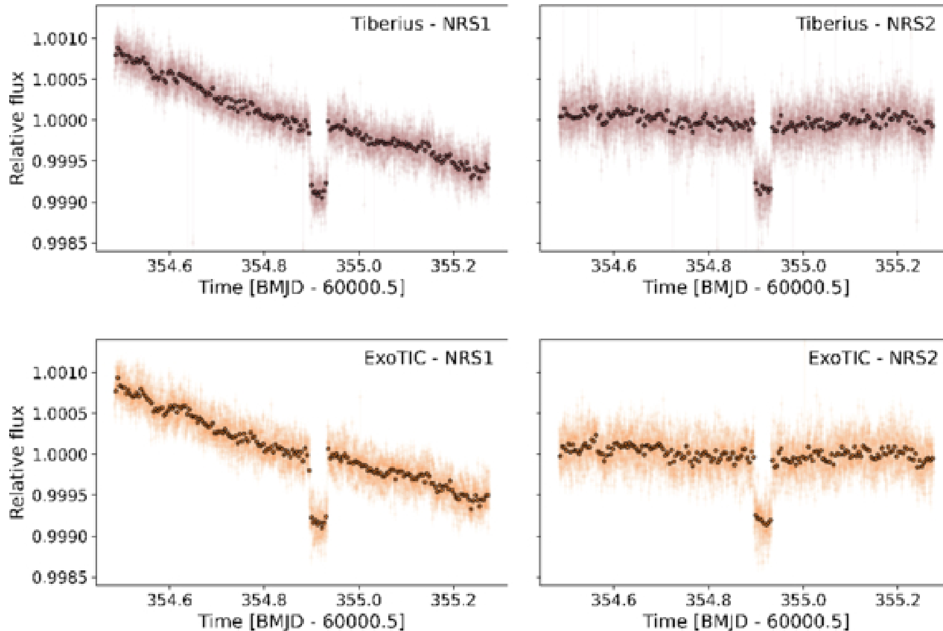
Figure 17. from Rafael Luque et al 2025 Astron. J. 170 doi:10.3847/1538-3881/addb40 https://dx.doi.org/10.3847/1538-3881/addb40 © 2025. The Author(s). Published by the American Astronomical Society.
