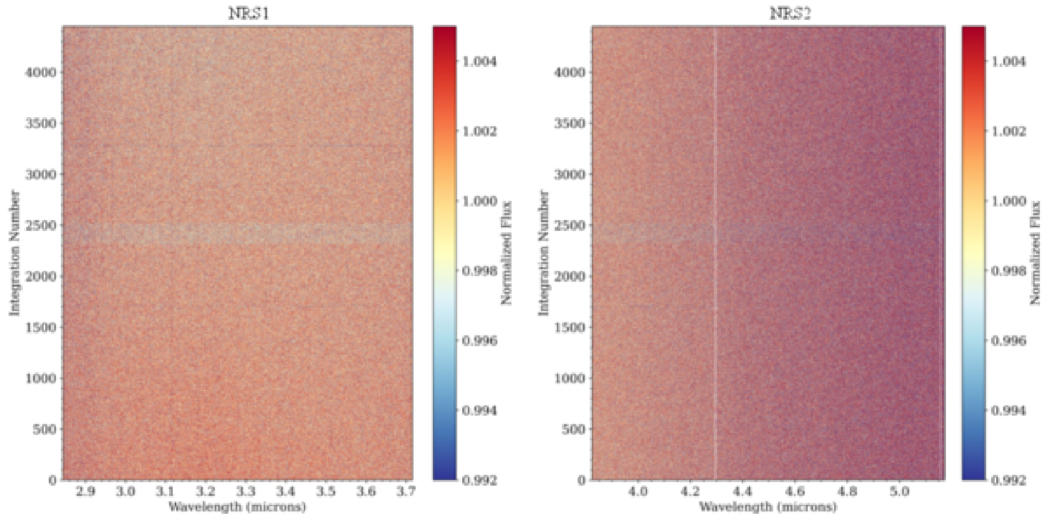
Figure 16. from Rafael Luque et al 2025 Astron. J. 170 doi:10.3847/1538-3881/addb40 https://dx.doi.org/10.3847/1538-3881/addb40 © 2025. The Author(s). Published by the American Astronomical Society.
