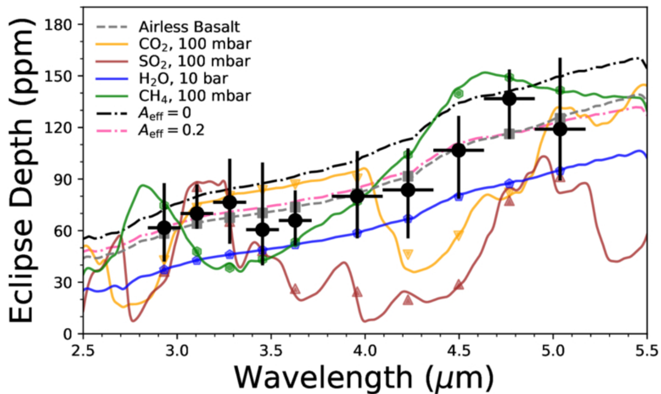
Figure 13. from Rafael Luque et al 2025 Astron. J. 170 doi:10.3847/1538-3881/addb40 https://dx.doi.org/10.3847/1538-3881/addb40 © 2025. The Author(s). Published by the American Astronomical Society.
