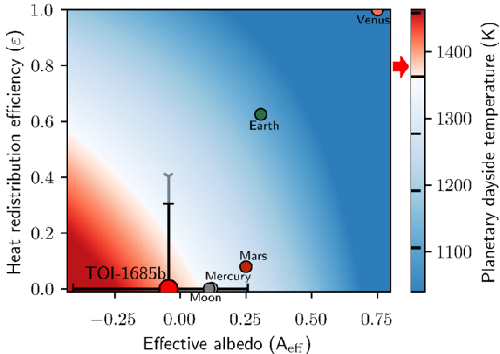
Figure 12. from Rafael Luque et al 2025 Astron. J. 170 doi:10.3847/1538-3881/addb40 https://dx.doi.org/10.3847/1538-3881/addb40 © 2025. The Author(s). Published by the American Astronomical Society.
