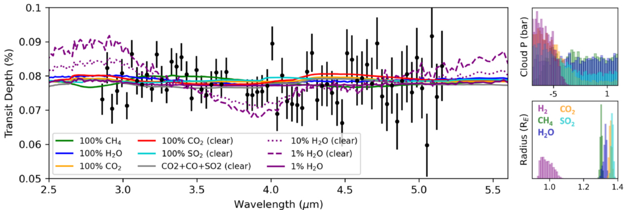
Figure 11. from Rafael Luque et al 2025 Astron. J. 170 doi:10.3847/1538-3881/addb40 https://dx.doi.org/10.3847/1538-3881/addb40 © 2025. The Author(s). Published by the American Astronomical Society.
