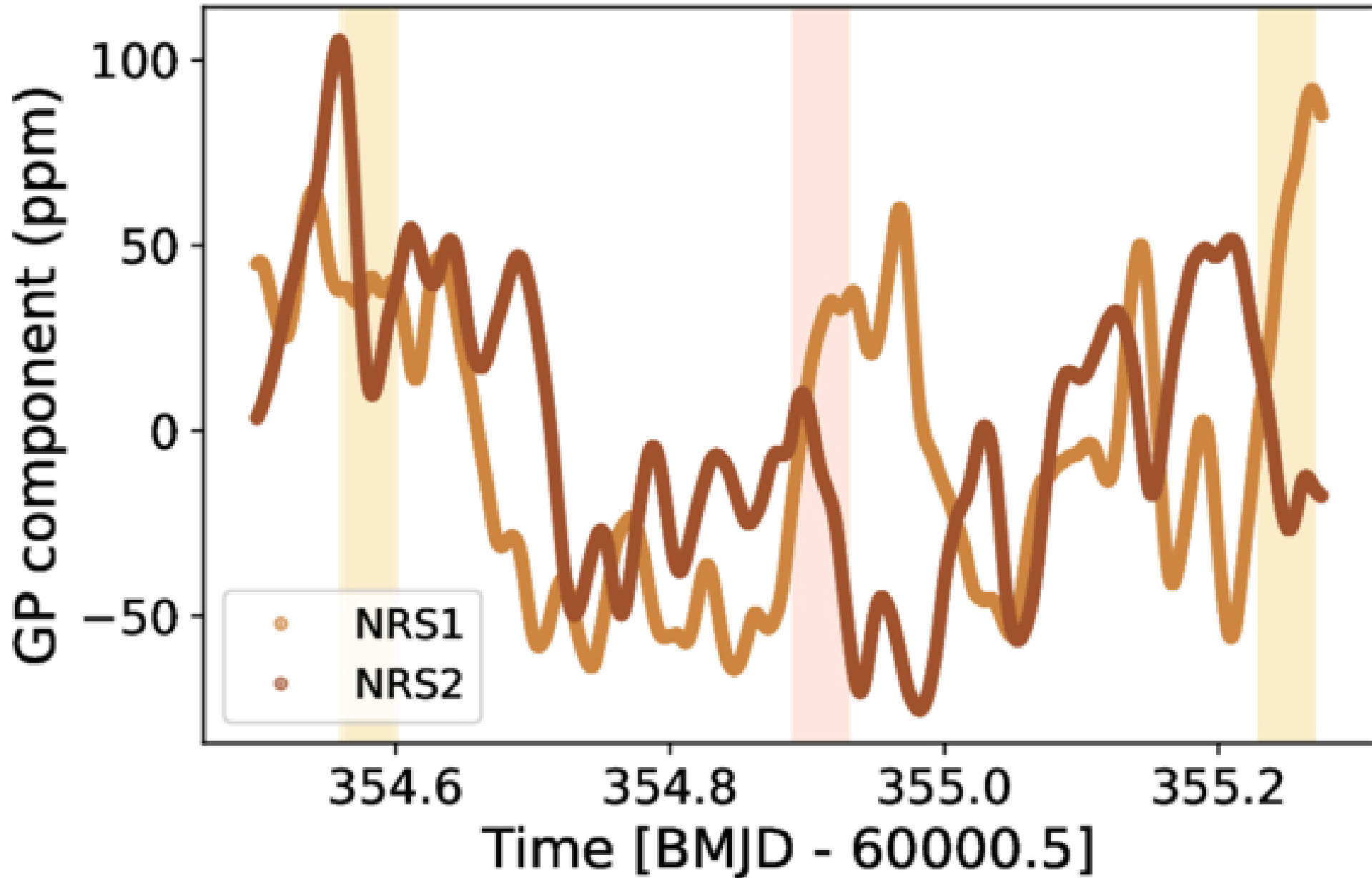
Figure 10. from Rafael Luque et al 2025 Astron. J. 170 doi:10.3847/1538-3881/addb40 https://dx.doi.org/10.3847/1538-3881/addb40 © 2025. The Author(s). Published by the American Astronomical Society.
