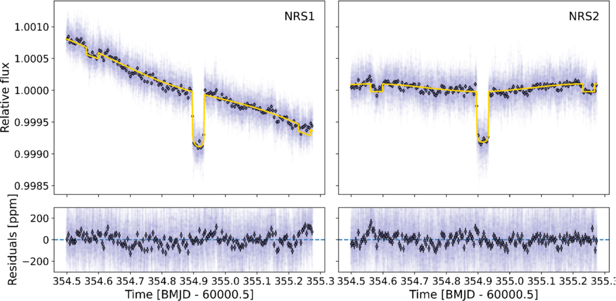
Figure 1. from Rafael Luque et al 2025 Astron. J. 170 doi:10.3847/1538-3881/addb40 https://dx.doi.org/10.3847/1538-3881/addb40 © 2025. The Author(s). Published by the American Astronomical Society.
