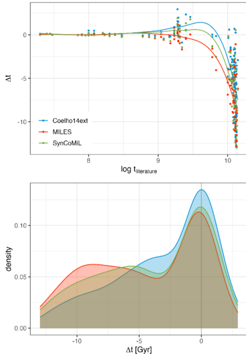
Figure 9. from Randa Asa'd et al 2025 Astron. J. 170 doi:10.3847/1538-3881/addaad https://dx.doi.org/10.3847/1538-3881/addaad © 2025. The Author(s). Published by the American Astronomical Society.
