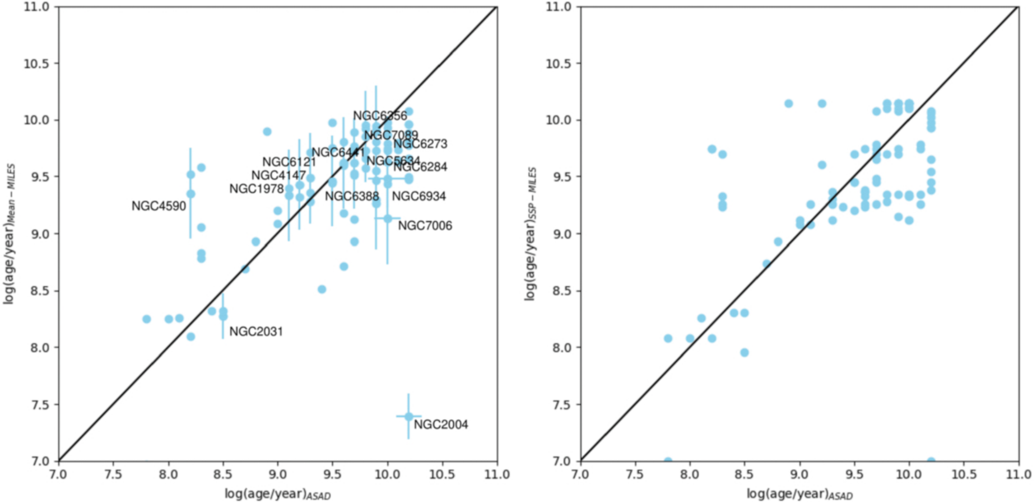
Figure 7. from Randa Asa'd et al 2025 Astron. J. 170 doi:10.3847/1538-3881/addaad https://dx.doi.org/10.3847/1538-3881/addaad © 2025. The Author(s). Published by the American Astronomical Society.
