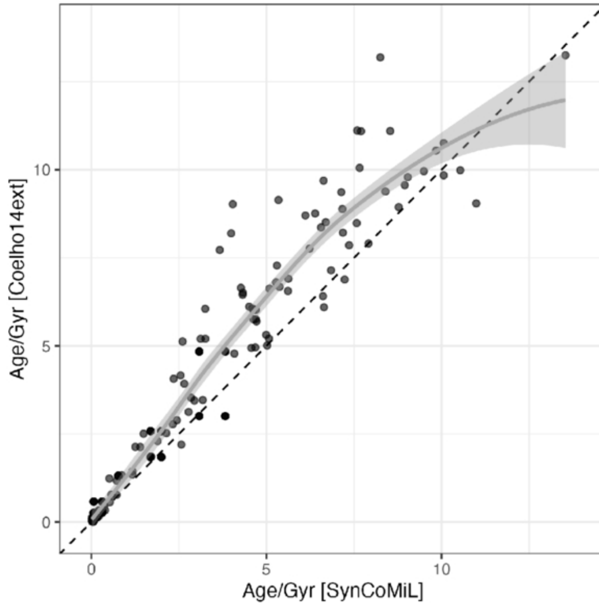
Figure 6. from Randa Asa'd et al 2025 Astron. J. 170 doi:10.3847/1538-3881/addaad https://dx.doi.org/10.3847/1538-3881/addaad © 2025. The Author(s). Published by the American Astronomical Society.
