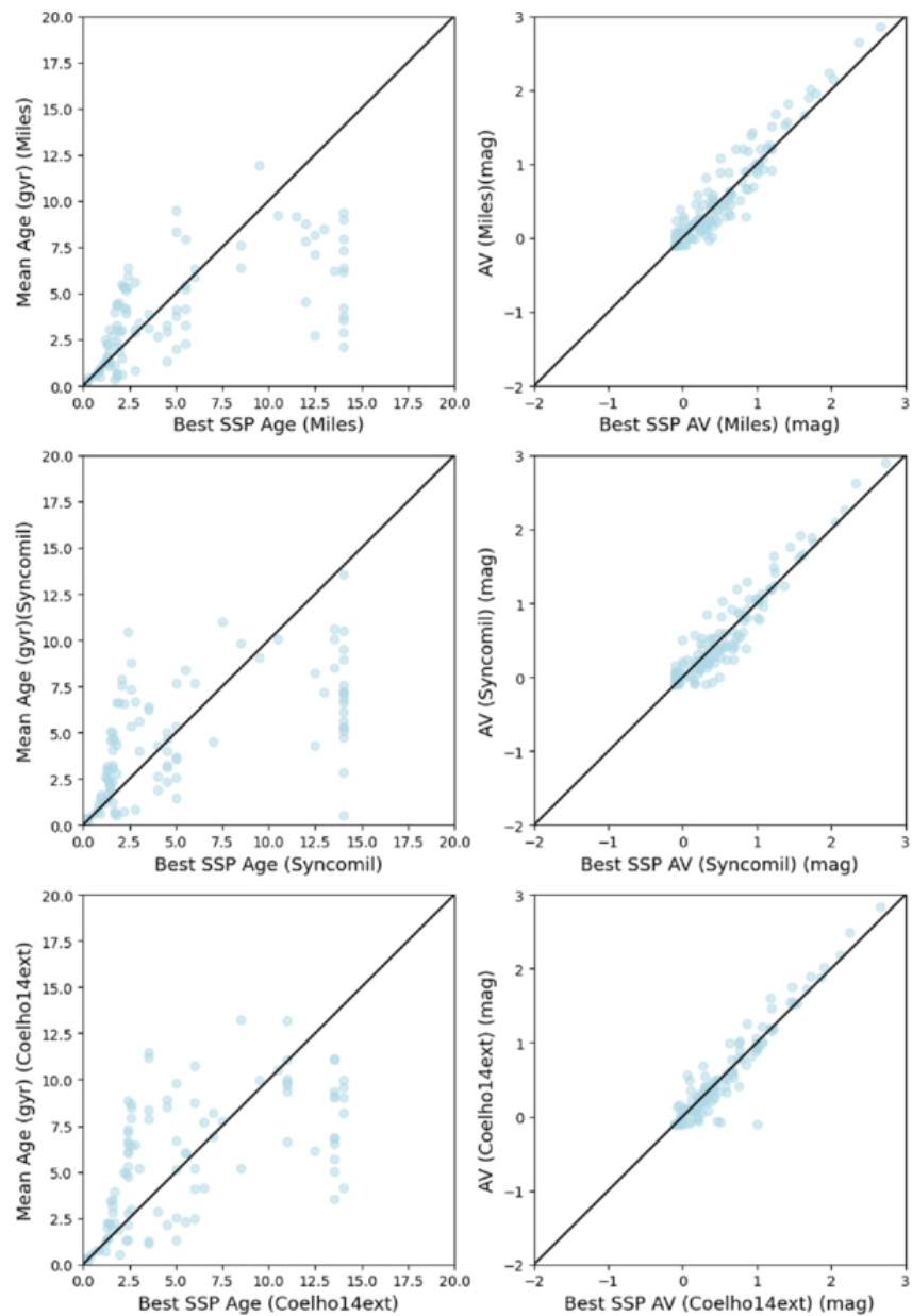
Figure 5. from Randa Asa'd et al 2025 Astron. J. 170 doi:10.3847/1538-3881/addaad https://dx.doi.org/10.3847/1538-3881/addaad © 2025. The Author(s). Published by the American Astronomical Society.
