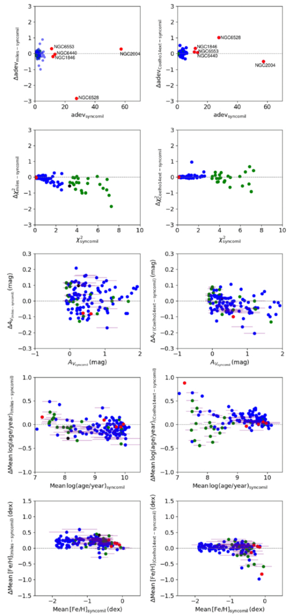
Figure 3. from Randa Asa'd et al 2025 Astron. J. 170 doi:10.3847/1538-3881/addaad https://dx.doi.org/10.3847/1538-3881/addaad © 2025. The Author(s). Published by the American Astronomical Society.
