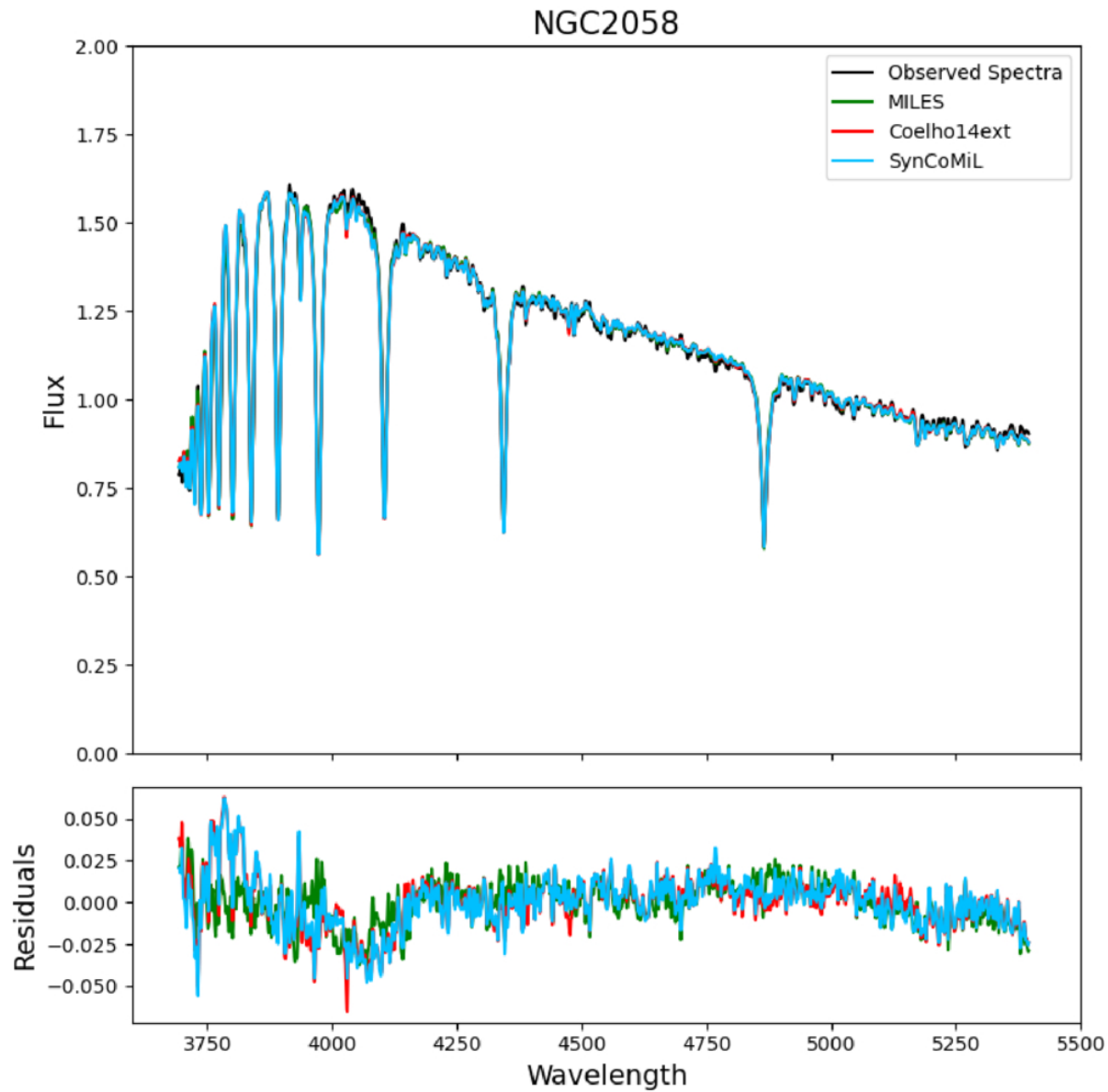
Figure 2. Spectral fits for star clusters in our sample. from Randa Asa'd et al 2025 Astron. J. 170 doi:10.3847/1538-3881/addaad https://dx.doi.org/10.3847/1538-3881/addaad © 2025. The Author(s). Published by the American Astronomical Society.
