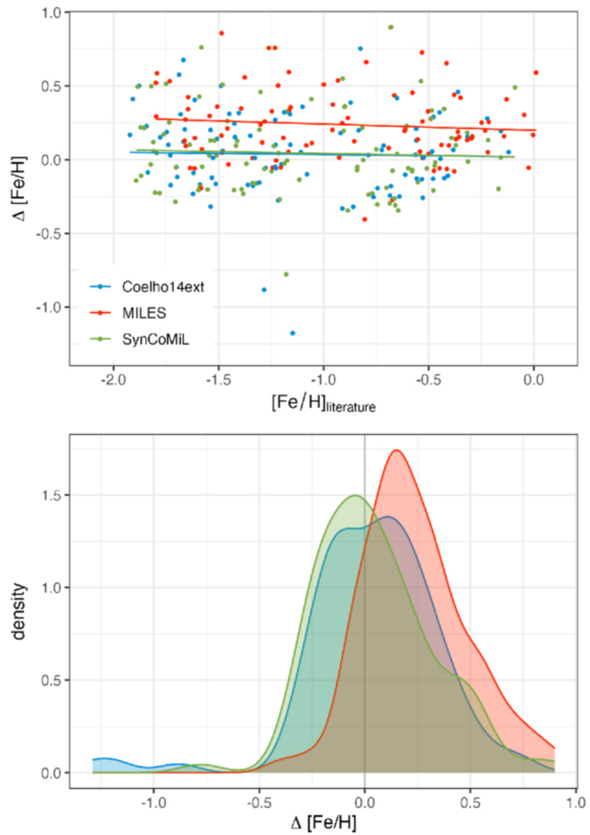
Figure 10. from Randa Asa'd et al 2025 Astron. J. 170 doi:10.3847/1538-3881/addaad https://dx.doi.org/10.3847/1538-3881/addaad © 2025. The Author(s). Published by the American Astronomical Society.
