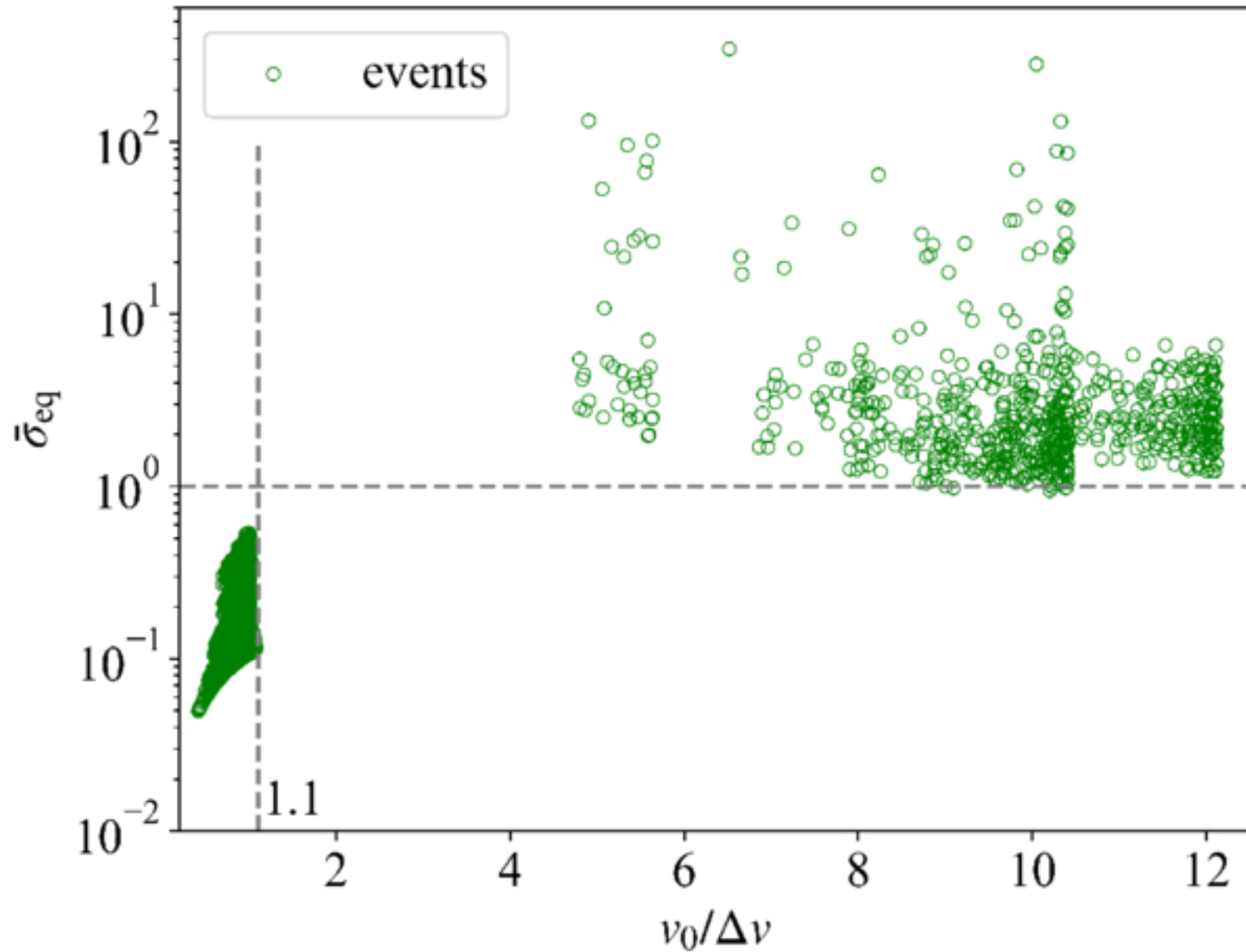
Figure 8. from Jian Chen et al 2025 Astron. J. 170 doi:10.3847/1538-3881/add937 https://dx.doi.org/10.3847/1538-3881/add937 © 2025. The Author(s). Published by the American Astronomical Society.
