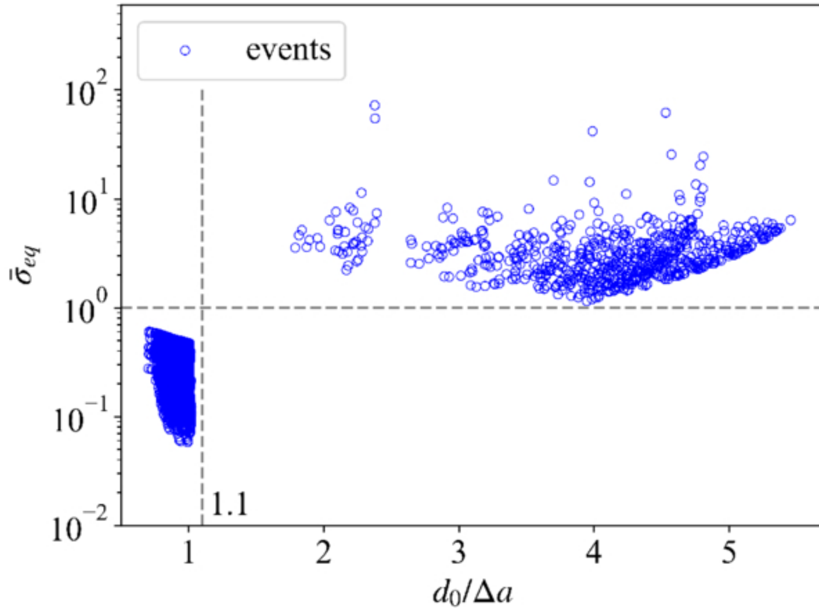
Figure 7. from Jian Chen et al 2025 Astron. J. 170 doi:10.3847/1538-3881/add937 https://dx.doi.org/10.3847/1538-3881/add937 © 2025. The Author(s). Published by the American Astronomical Society.
