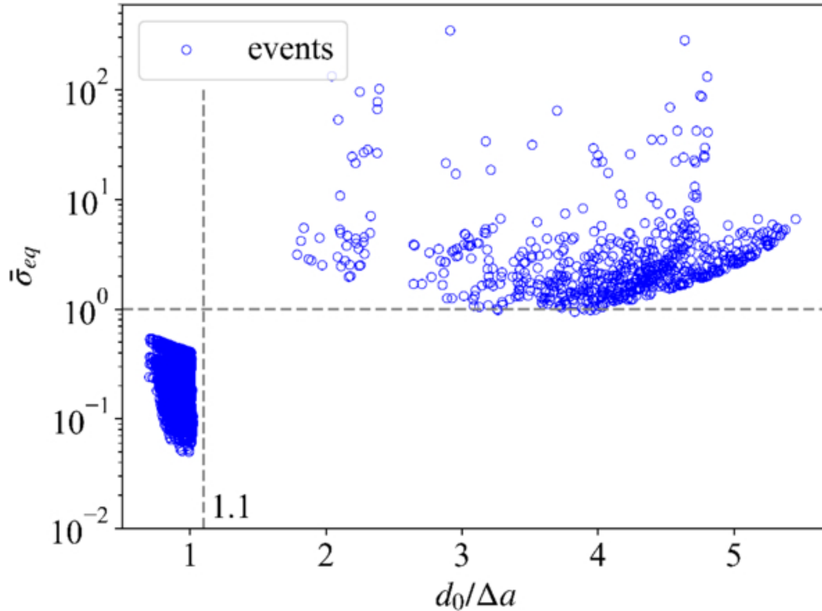
Figure 6. from Jian Chen et al 2025 Astron. J. 170 doi:10.3847/1538-3881/add937 https://dx.doi.org/10.3847/1538-3881/add937 © 2025. The Author(s). Published by the American Astronomical Society.
