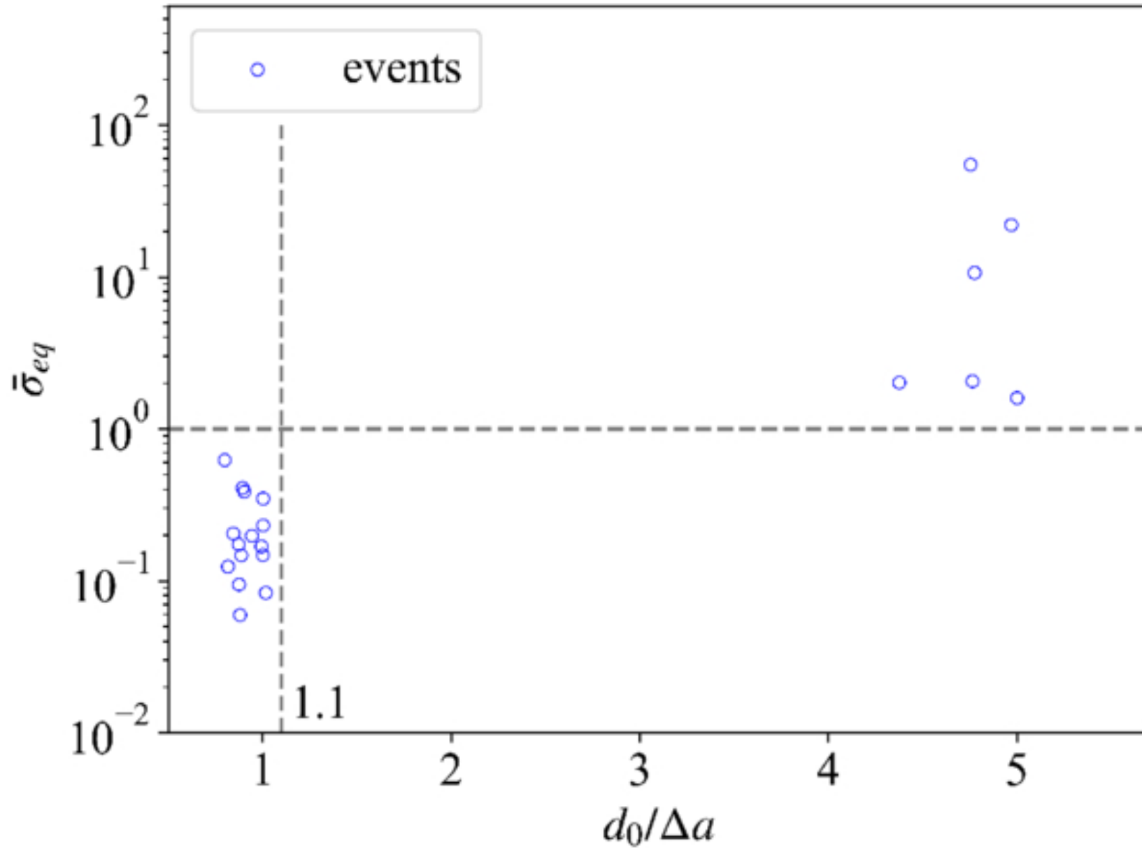
Figure 3. from Jian Chen et al 2025 Astron. J. 170 doi:10.3847/1538-3881/add937 https://dx.doi.org/10.3847/1538-3881/add937 © 2025. The Author(s). Published by the American Astronomical Society.
