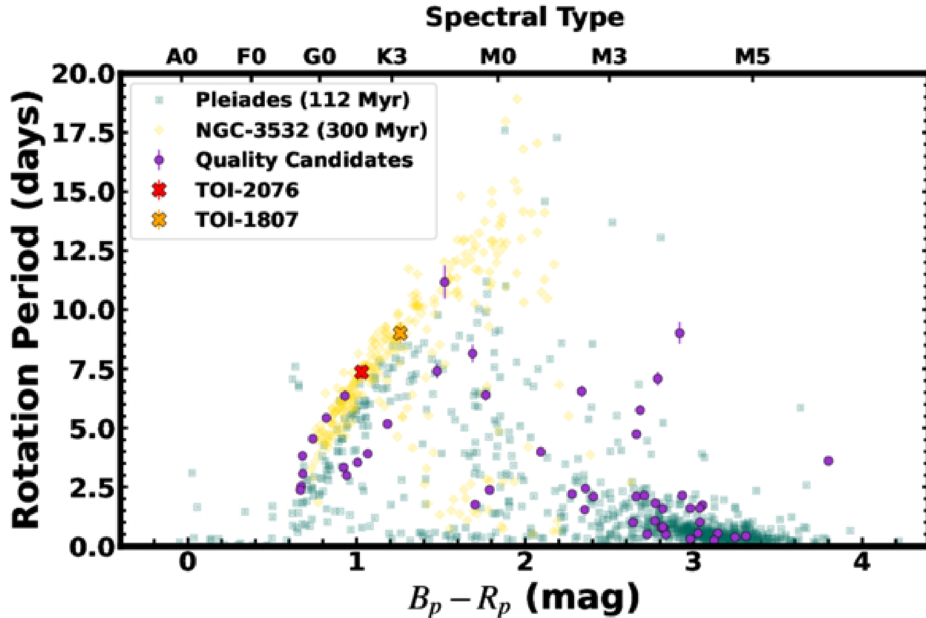
Figure 5. from Madyson G. Barber et al 2025 Astron. J. 170 doi:10.3847/1538-3881/add7db https://dx.doi.org/10.3847/1538-3881/add7db © 2025. The Author(s). Published by the American Astronomical Society.
